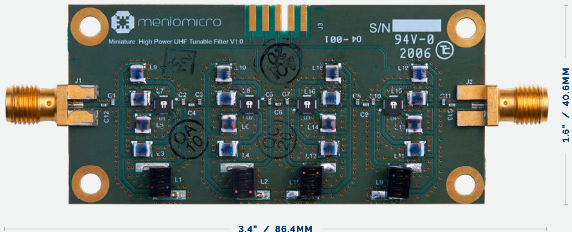
FIG. 2 Filter PCB
